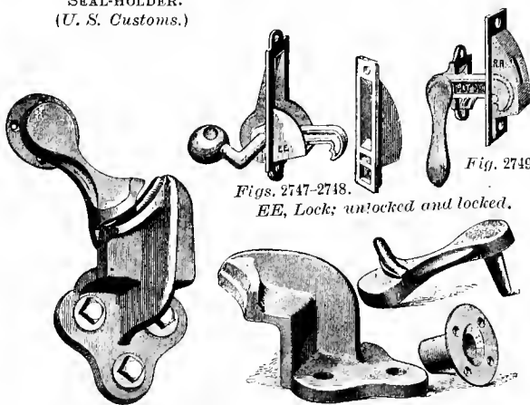
Fig. 2752. Howard Lock.
